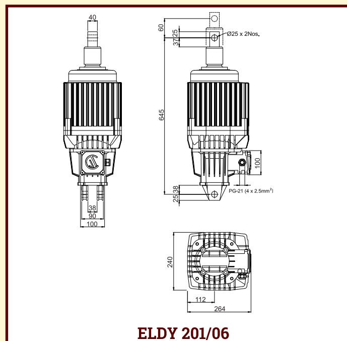
ELECTRO-HYDRAULIC THRUSTER MODEL ELDY 201/06
