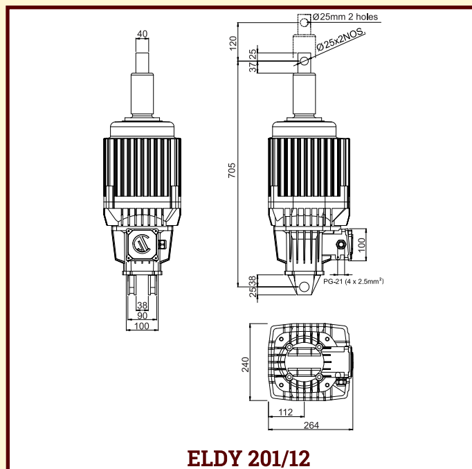
ELECTRO-HYDRAULIC THRUSTER MODEL ELDY 201/12
