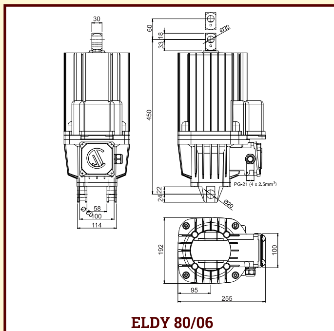
ELECTRO-HYDRAULIC THRUSTER MODEL ELDY 80/06
