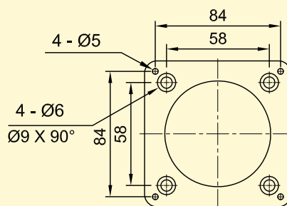
Mounting Dimension
