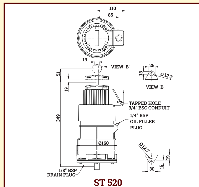
ELECTRO-HYDRAULIC THRUSTER MODEL ST 520
