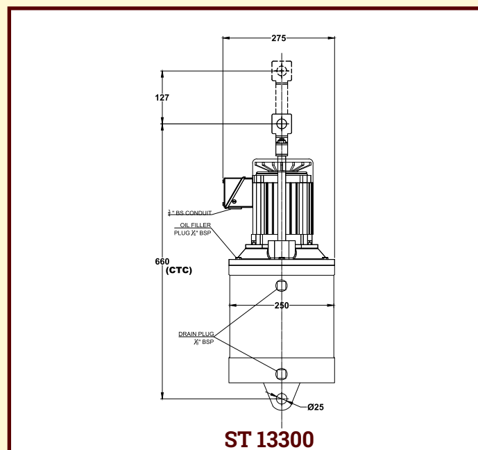
ELECTRO-HYDRAULIC THRUSTER MODEL ST 13300
