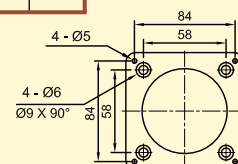
Mounting Dimension
